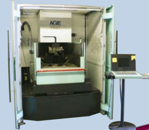
2002 AGIE Wire Electric Discharge Machine
